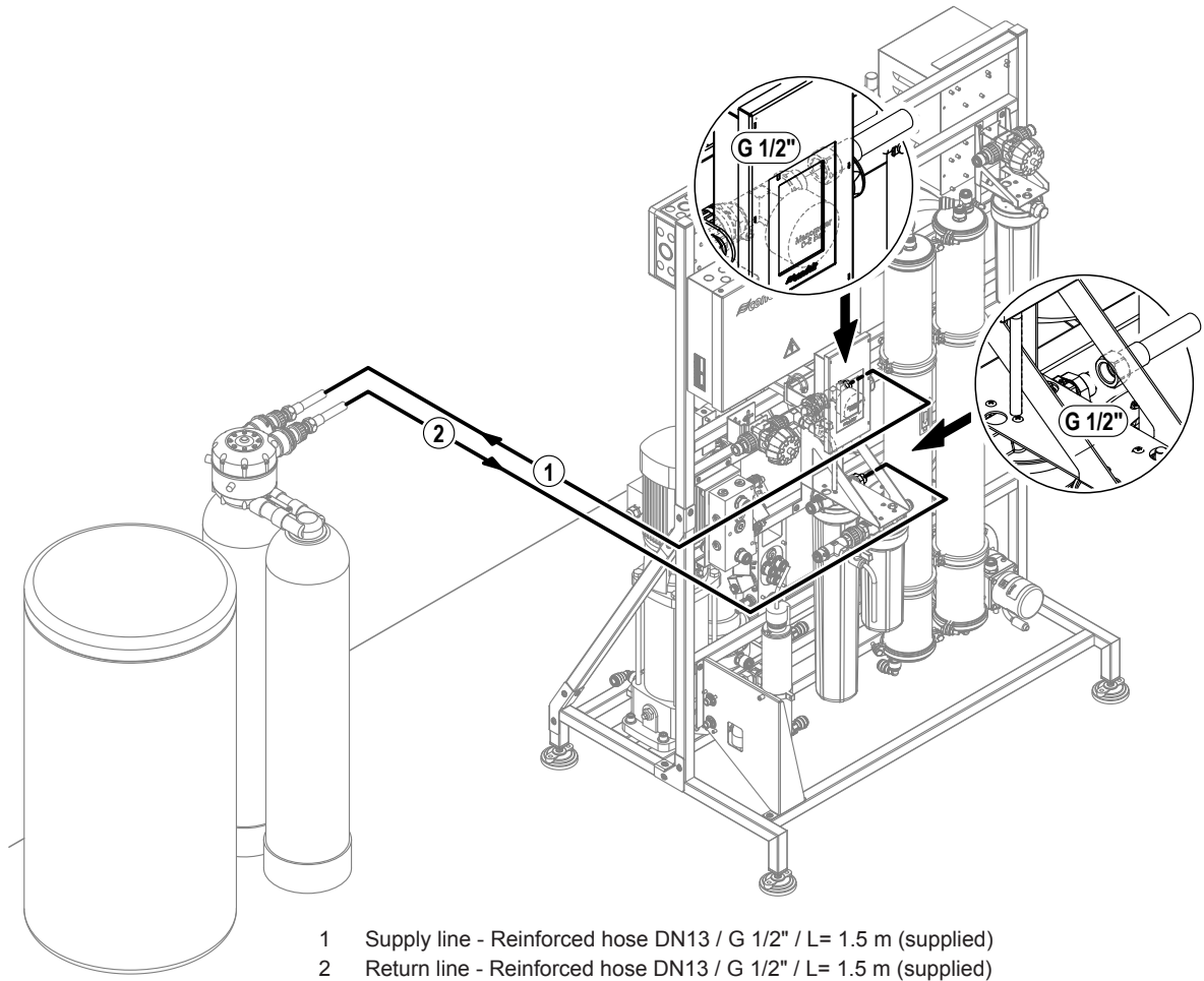
Fig. 12: Connecting the water softener to the Condair Vita Power (image shows Condair Vita Power RO-DI-CO-UV-HP 500 l/hr)
