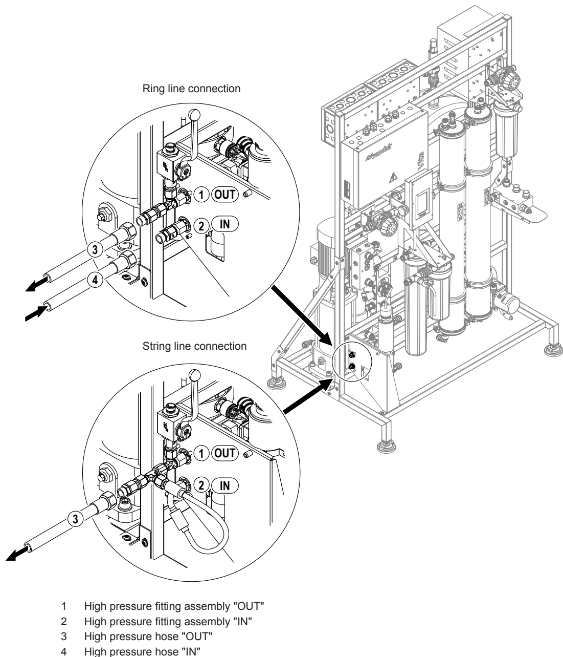
Fig. 15: Connecting the high pressure lines to the Condair Vita Power (image shows Condair Vita Power RO-DI-CO-UV-HP 500 l/hr)
