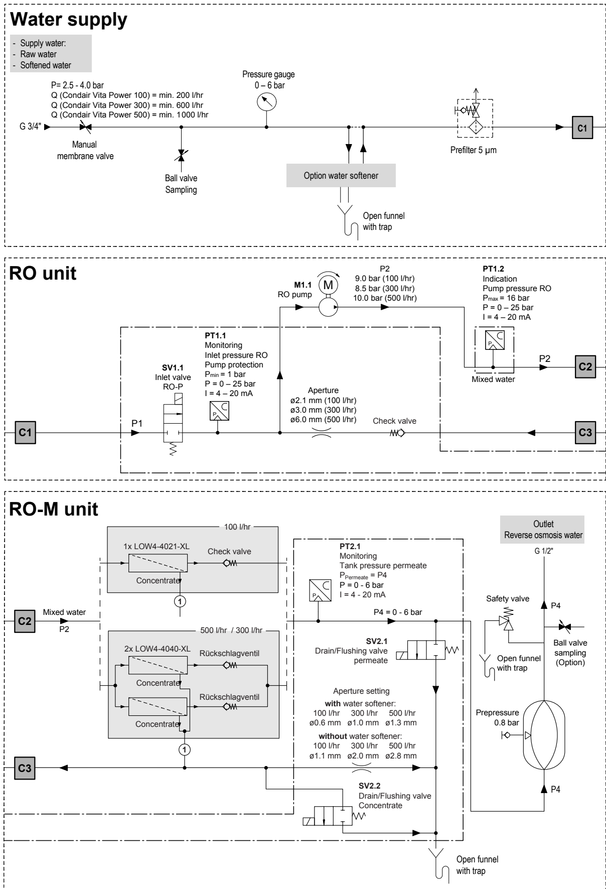
Fig. 27: Hydraulic diagram Condair Vita Power RO
