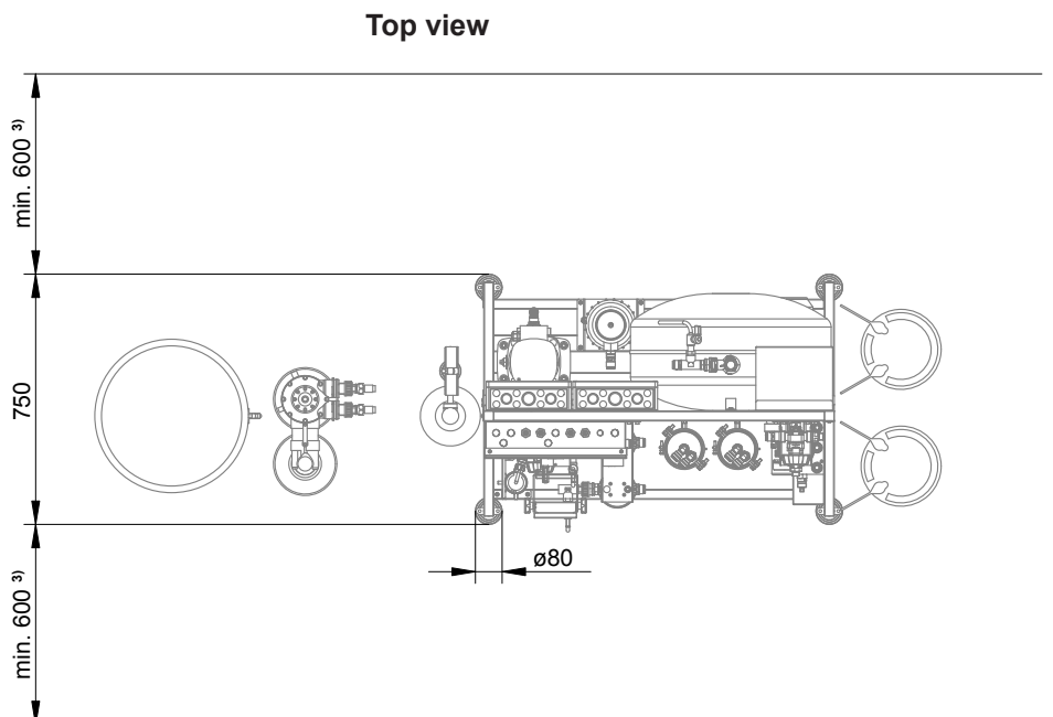
Fig. 5: System dimensions Vita Power RO-DI-CO-UV-HP (dimensions in mm)
